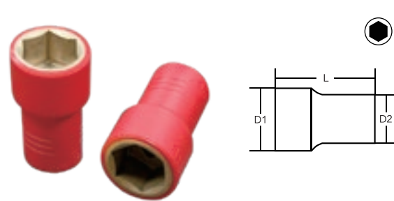
3/8"双色绝缘防爆公制套筒 3/8"INSULATED EXPLOSION-PROOF HEXAGON SOCKETS
